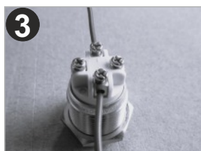
3 LED anschließen Connect LED
