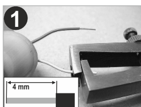
1 Draht abisolieren (4 mm) Strip the wire (4 mm)
